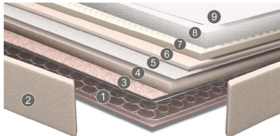
1. Ressort continu Multielastic Nxt® 2. Encapsulage 3. Filtre thermo-bound 500 g 4. Confort System 12 mm, 5. Textile NT 17 g 6. Mousse 9 mm 7. Système Commodo® 21 mm 8. Couverture compacte 175 g 9. Tissu Stretch
